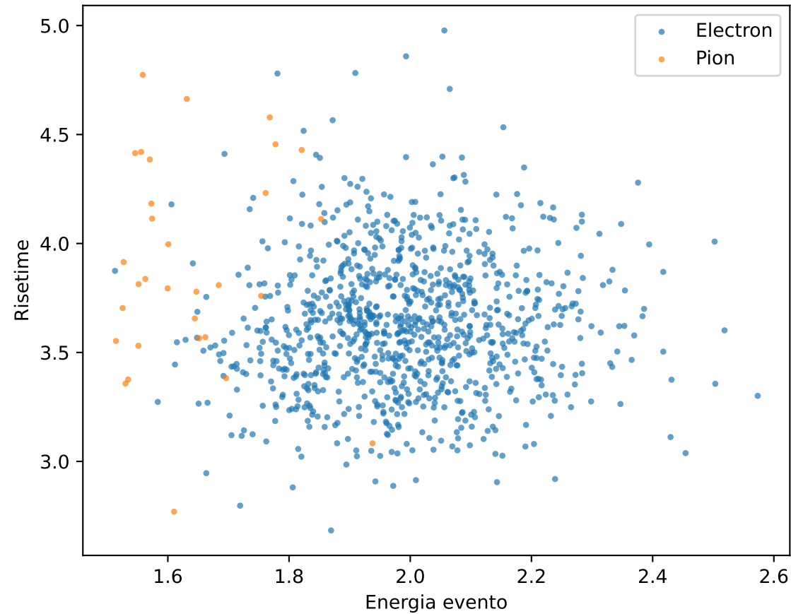
Scatter plot e/pi (cutted) 2.0GeV
