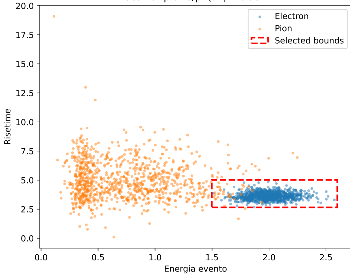
Scatter plot e/pi (all) 2.0GeV
